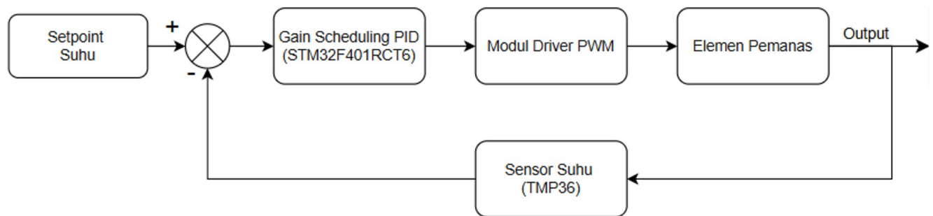
Diagram Blok Tertutup Gain Scheduling PID
