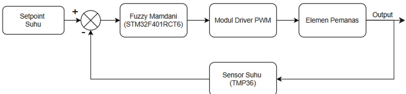
Diagram Blok Tertutup Fuzzy Mamdani
